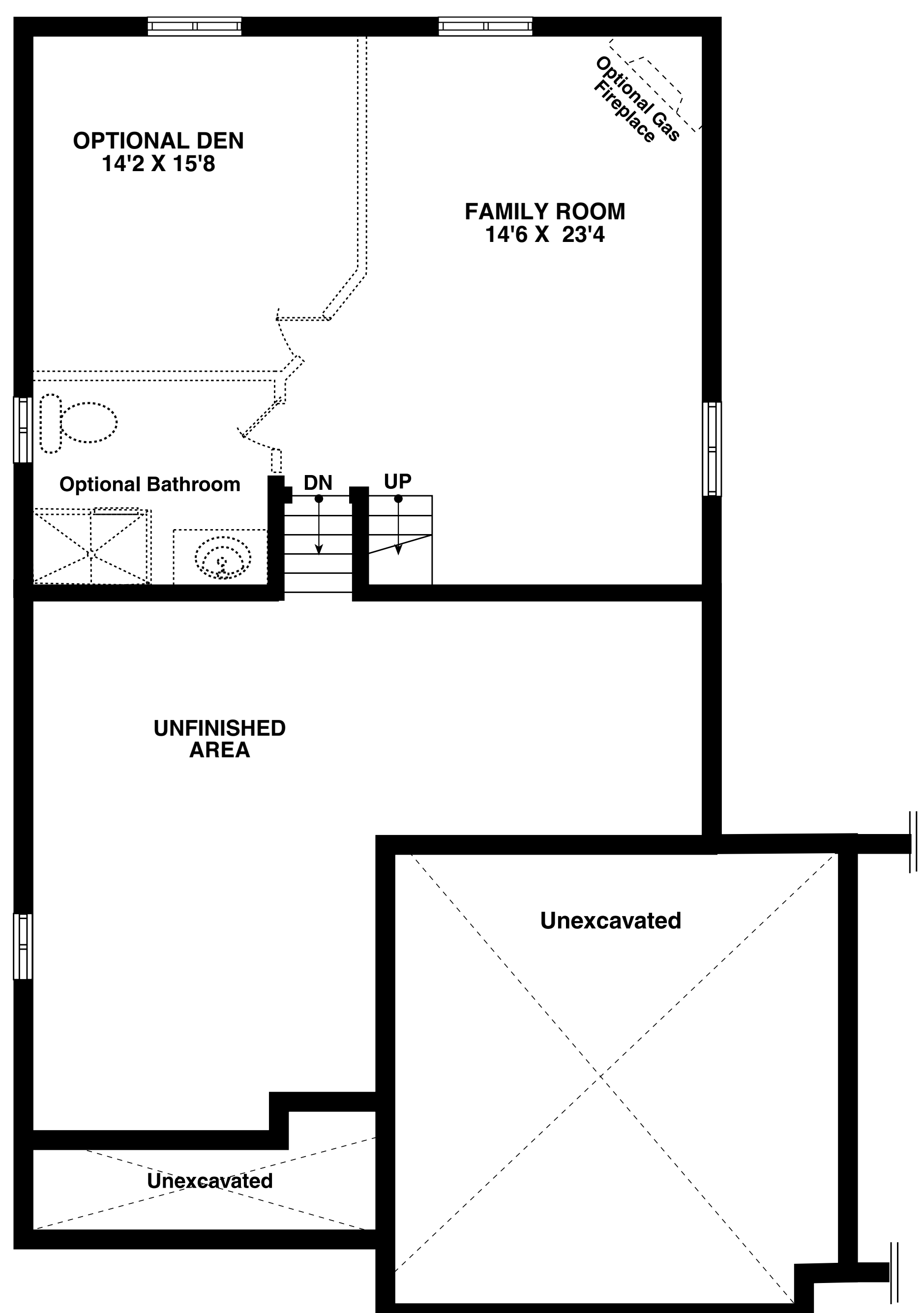
Basement Plan
